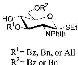
Figure 1: The C-3 and C-6 protecting groups used on the ethyl 2-deoxy-2-phthalimido-1- \beta -D-thio-glucosamine compounds subjected to epimerization.
