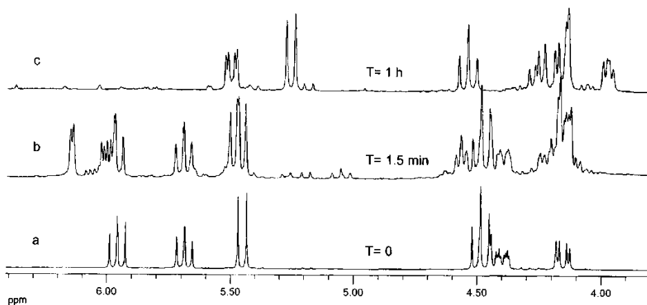
Figure 2: ^1\text{H} NMR spectra from the substitution of presynthesized triflate of 3 using \text{NaNO}_2 in \text{DMF-d}_7 . (a) T = 0 , synthesized triflate of compound 3 ; (b) T = 1.5 min, mixture of starting compound and the suggested intermediate nitrous acid ester; (c) T = 1 hr, only galacto epimer 11 is observed after collapse of the intermediate compound. For further information see text.
